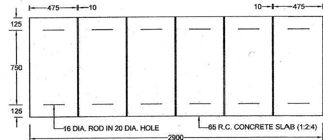
PLAN OF SLAB
