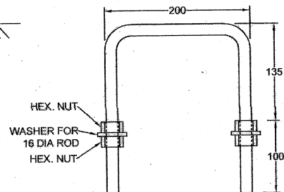
DETAILS OF LIFTING HANDLE
