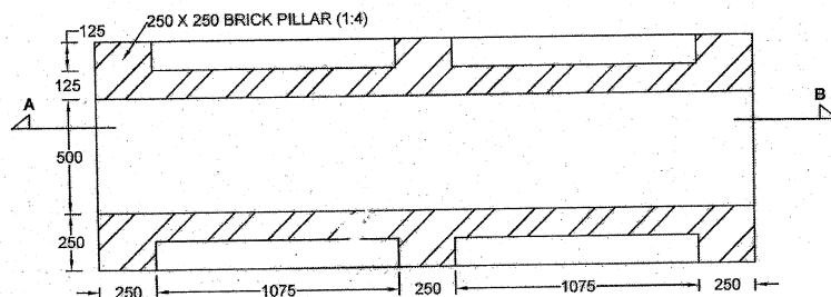
PLAN OF PROTECTION DUCT FOR CABLE JOINT
