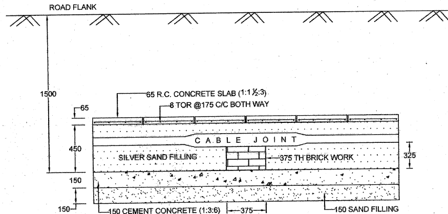
SECTION AT 'AB'
